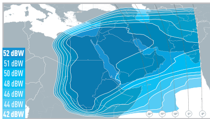
EUTELSAT 8 West B Eastern Africa coverage
