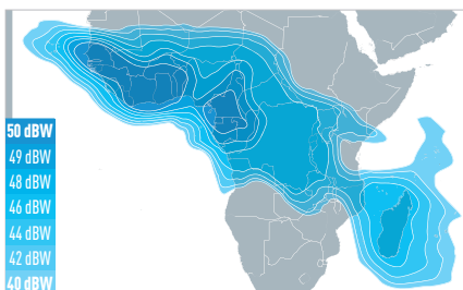
EUTELSAT 16A Africa coverage
