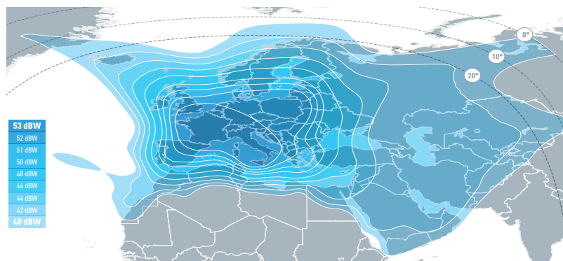
HOTBIRD 13F & 13G KU-BAND WIDEBEAM DOWNLINK COVERAGE
