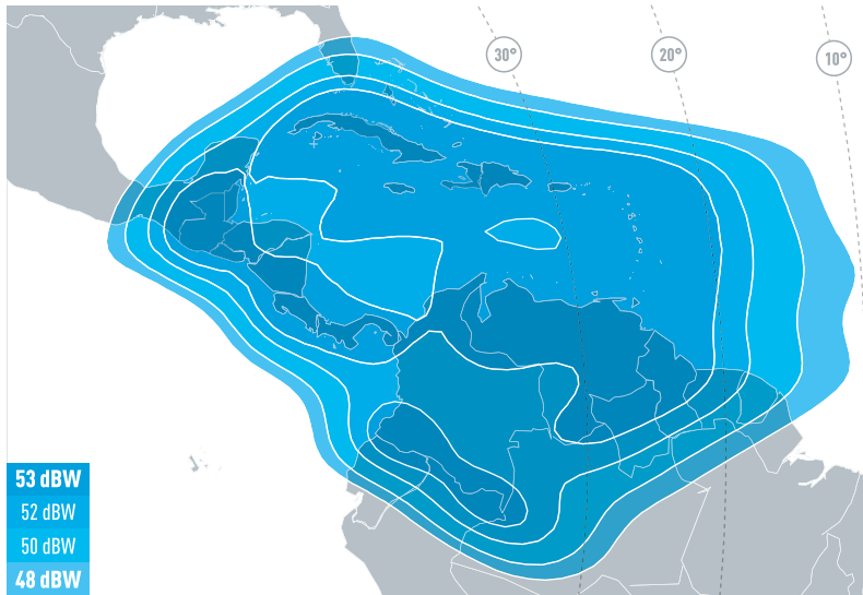
KU-BAND 5 CENTRAL AMERICA DOWNLINK COVERAGE
