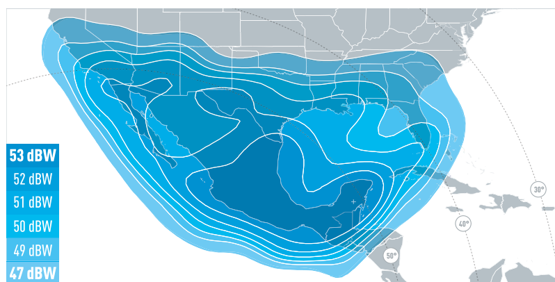
KU-BAND 1 MEXICO DOWNLINK COVERAGE
