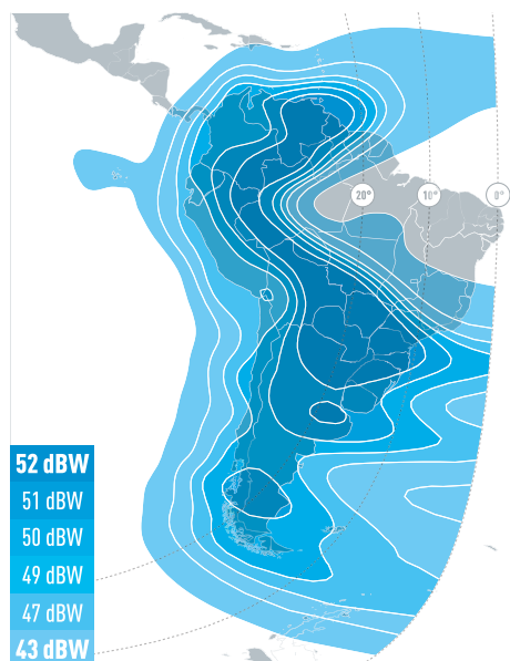
KU-BAND 3 SOUTH AMERICA DOWNLINK COVERAGE
