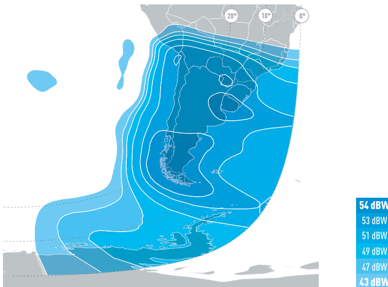
KU-BAND 6 SOUTHERN CONE DOWNLINK COVERAGE
