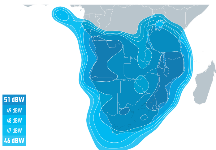
EUTELSAT 36D KU-BAND SOUTHERN AFRICA DOWNLINK COVERAGE
