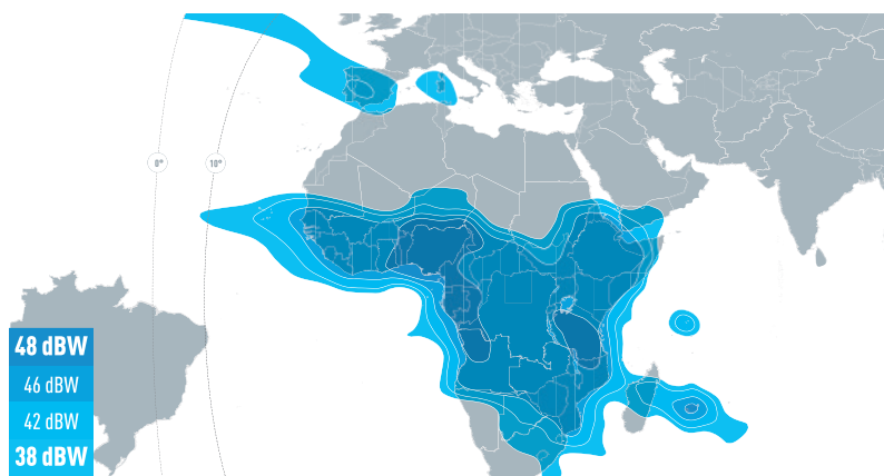
EUTELSAT 36D KU-BAND CENTRAL AFRICA DOWNLINK COVERAGE
