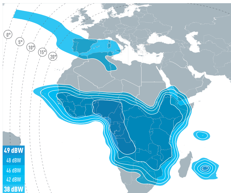
EUTELSAT 36C KU-BAND AFRICA DOWNLINK COVERAGE
